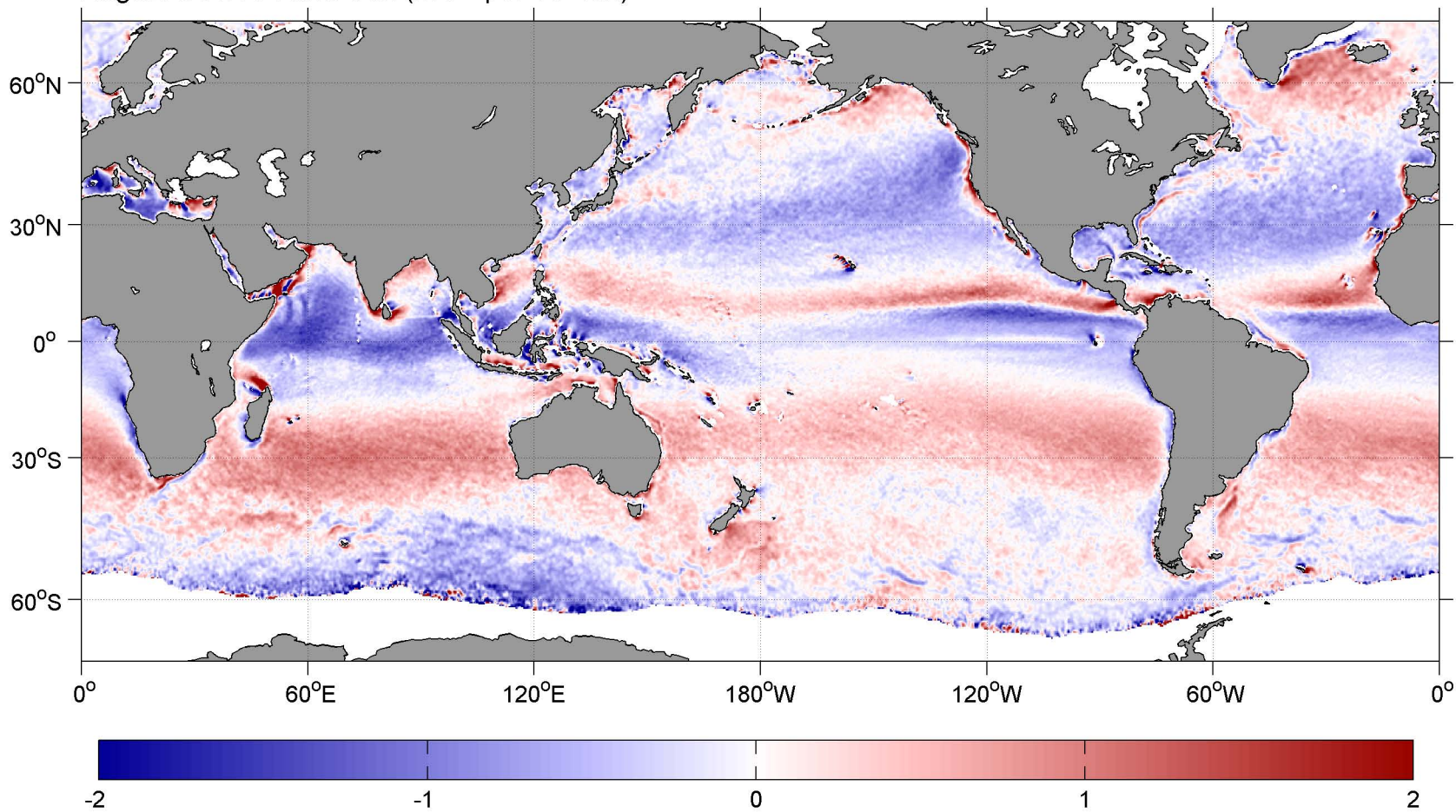
August SCOW Wind Curl ( \text{m s}^{-1} per 10^2 \text{ km} )
