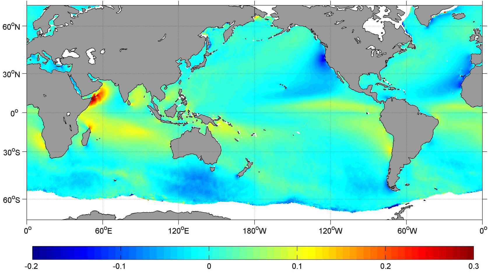
August SCOW Zonal Meridional Stress ( \text{N m}^{-2} )
