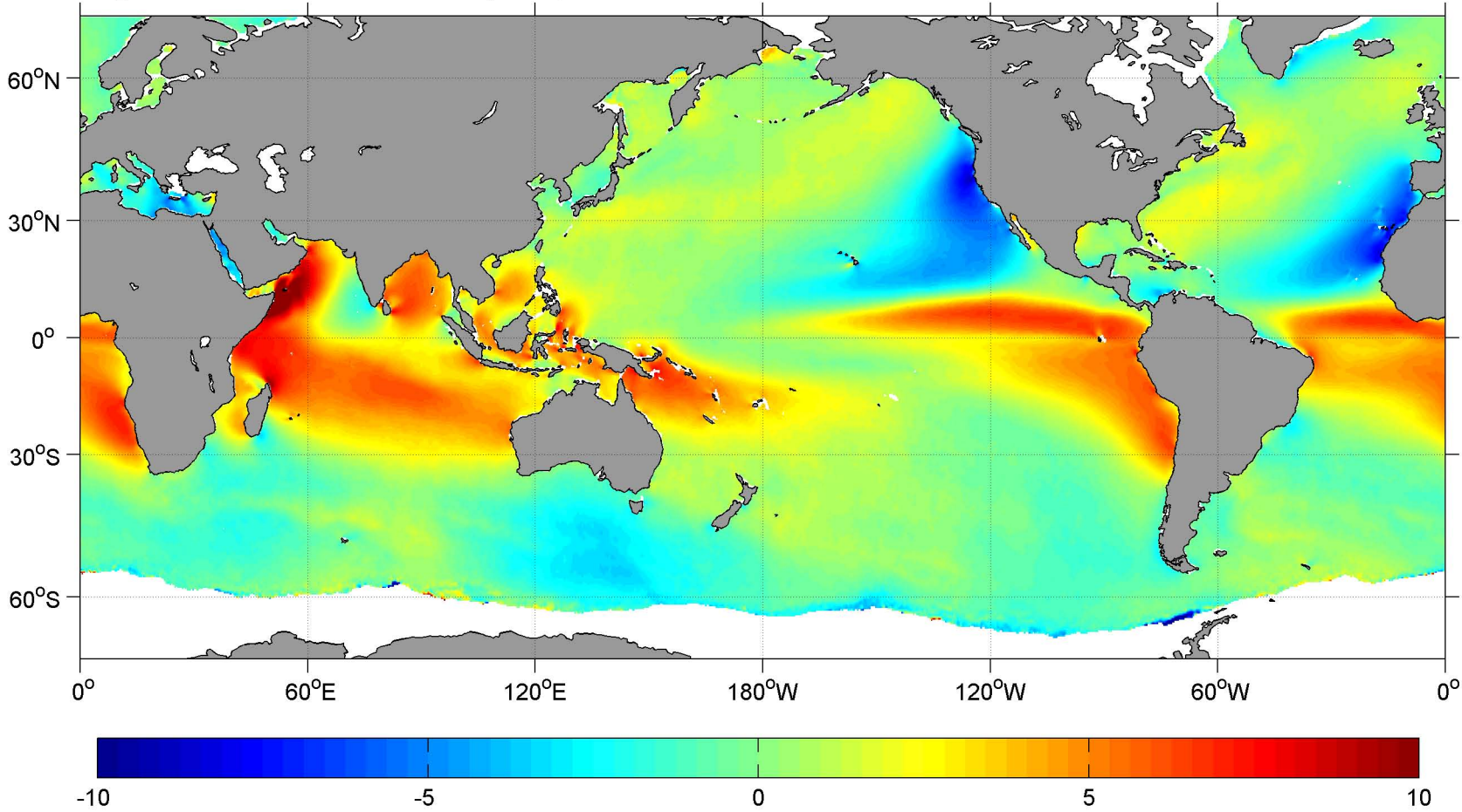
August SCOW Meridional Wind ( \text{m s}^{-1} )
