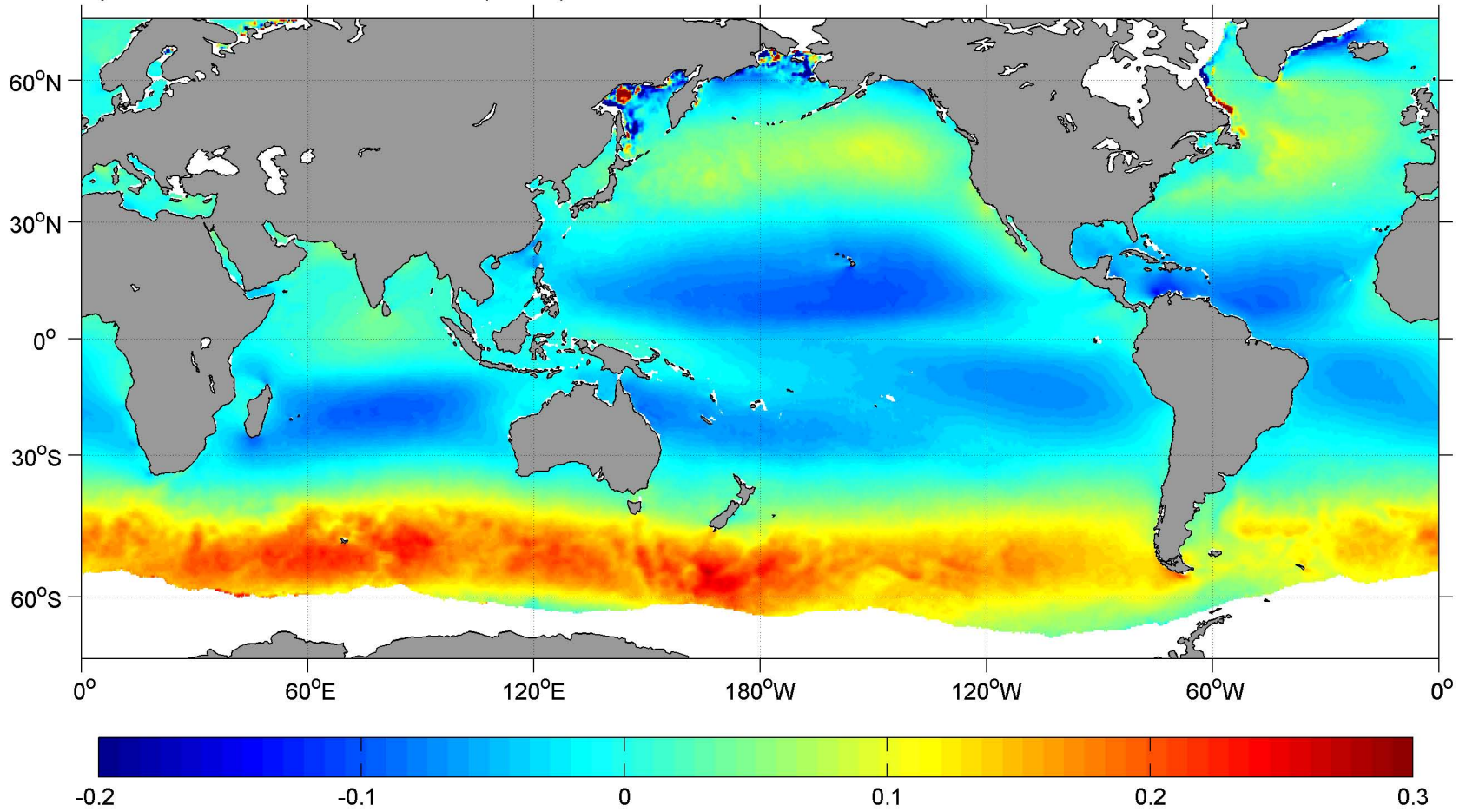
April SCOW Zonal Wind Stress ( \text{N m}^{-2} )
