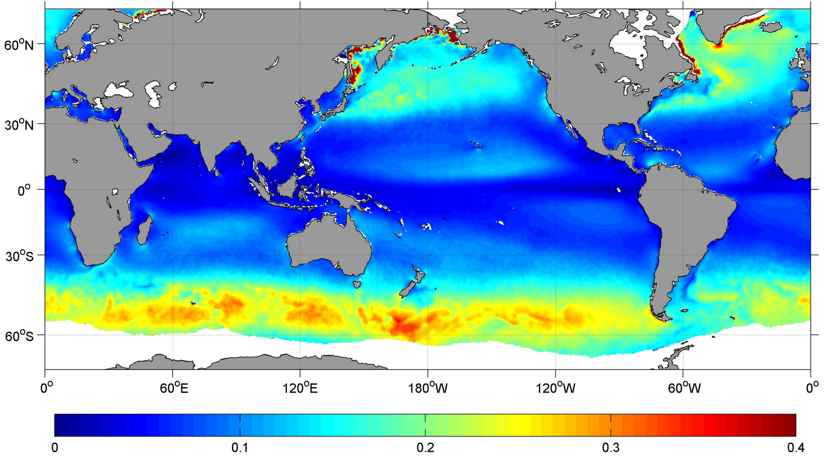
April SCOW Wind Stress Magnitude ( \text{N m}^{-2} )
