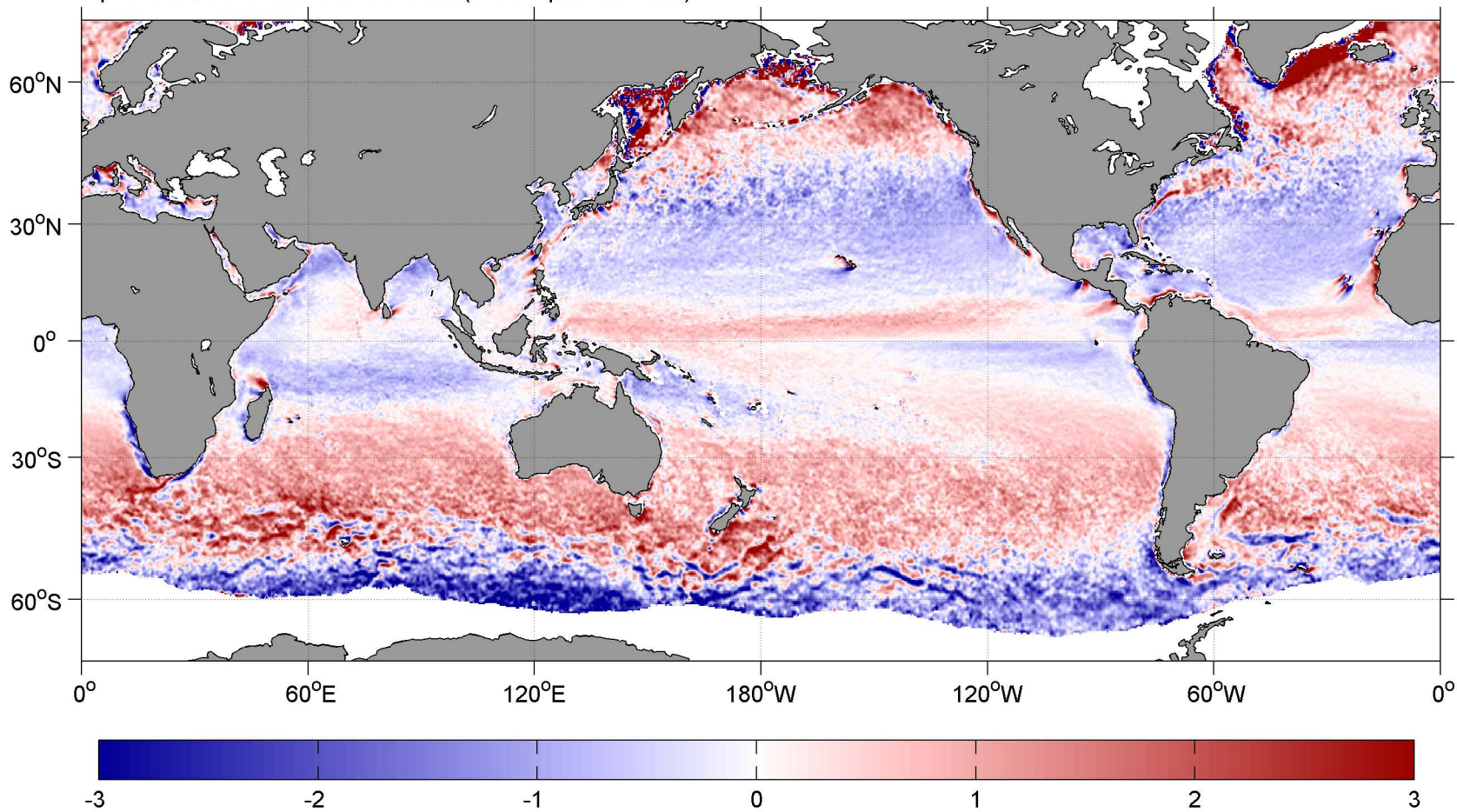
April SCOW Wind Stress Curl ( \text{N m}^{-2} per 10^4 \text{ km}^2 )
