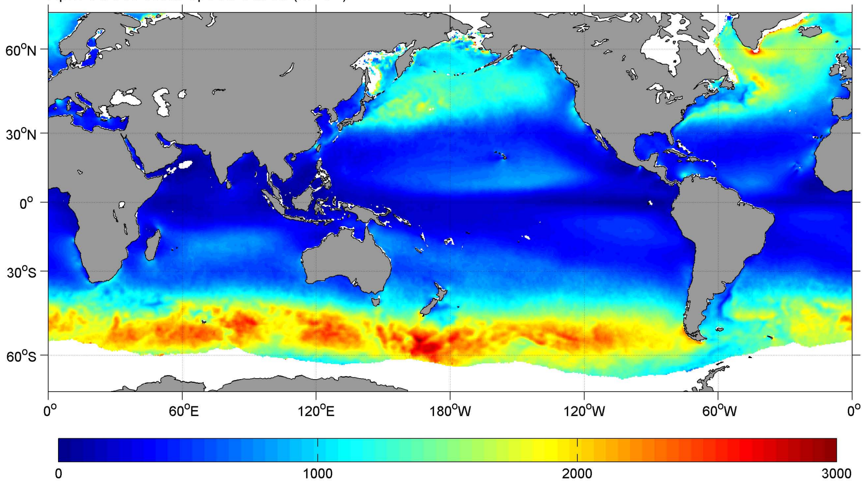
April SCOW Wind Speed Cubed ( \text{m}^3 \text{s}^{-3} )
