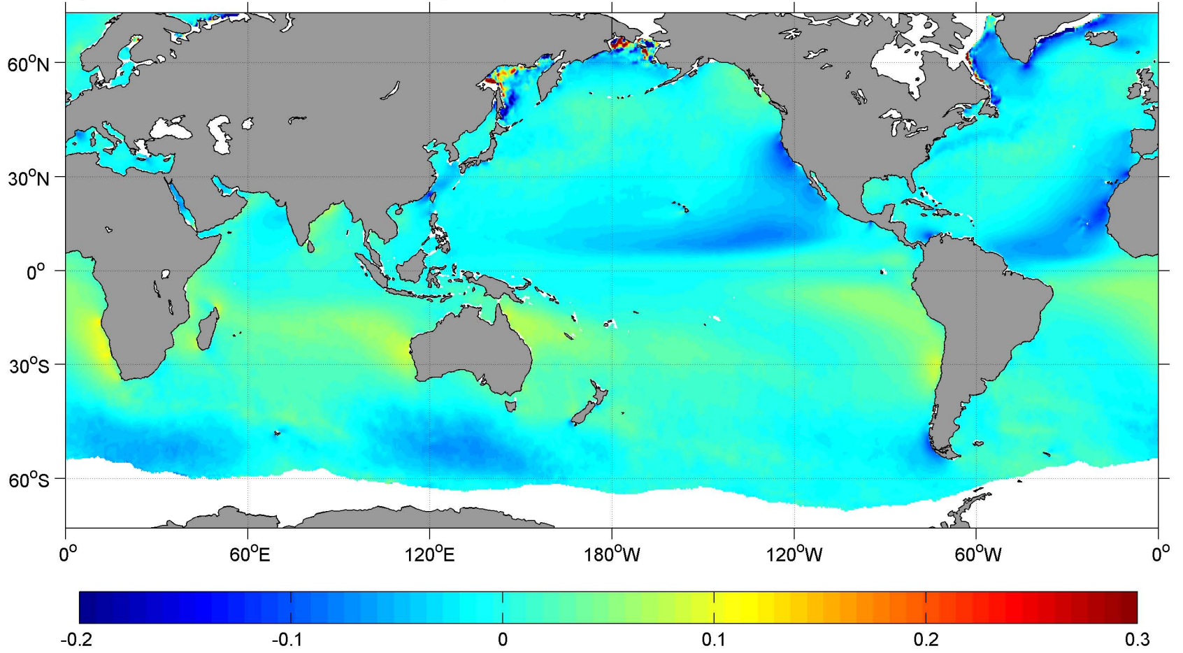
April SCOW Zonal Meridional Stress ( \text{N m}^{-2} )
